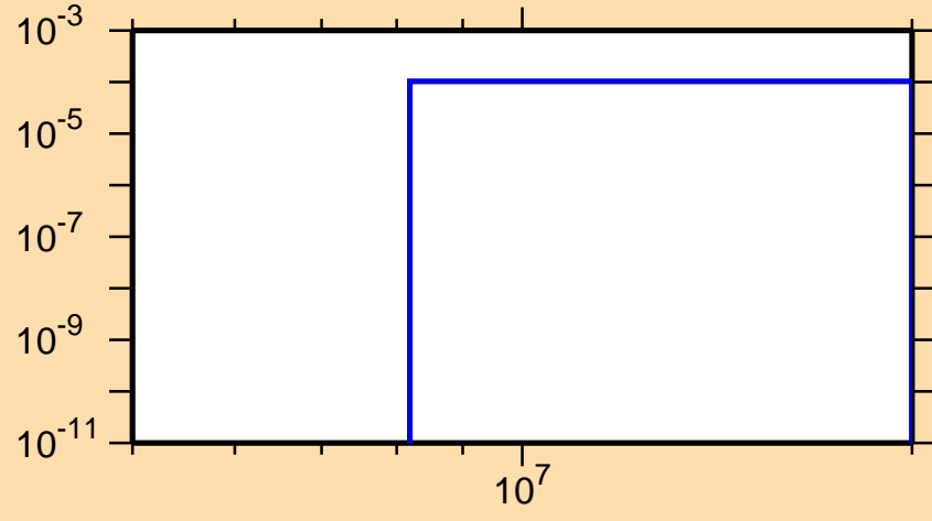
\sigma vs. E for ^{90}\text{Tc}(n,n\alpha)
