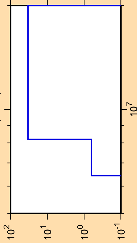
\Delta\sigma/\sigma vs. E for ^{90}\text{Tc}(n,n\alpha)
