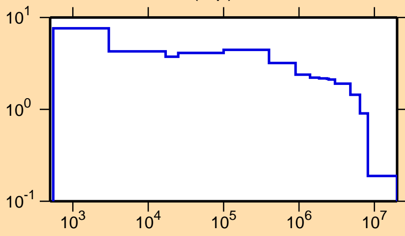
\sigma vs. E for ^{90}\text{Tc}(n,p)
