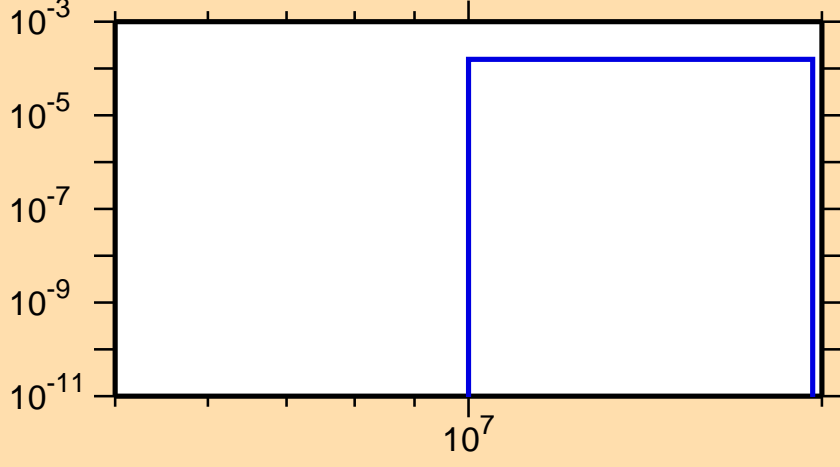
\sigma vs. E for ^{90}\text{Tc}(n,pd)
