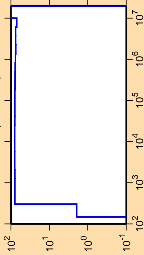
\Delta\sigma/\sigma vs. E for ^{90}\text{Tc}(n,\text{ncont.})
