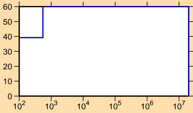
\Delta\sigma/\sigma vs. E for ^{90}\text{Tc}(n,ncont.)
