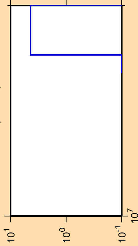
\Delta\sigma/\sigma vs. E for ^{90}\text{Tc}(n,2n\alpha)
