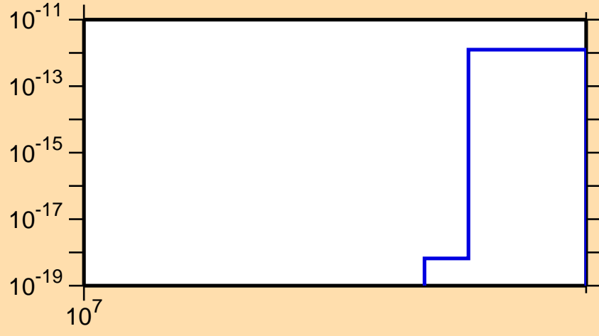
\sigma vs. E for ^{90}\text{Tc}(n,2n\alpha)
