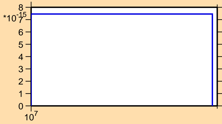
\sigma vs. E for ^{90}\text{Tc}(n,2n\alpha)
