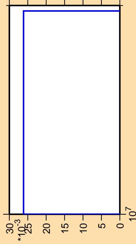
\Delta\sigma/\sigma vs. E for ^{90}\text{Tc}(n,2n\alpha)
