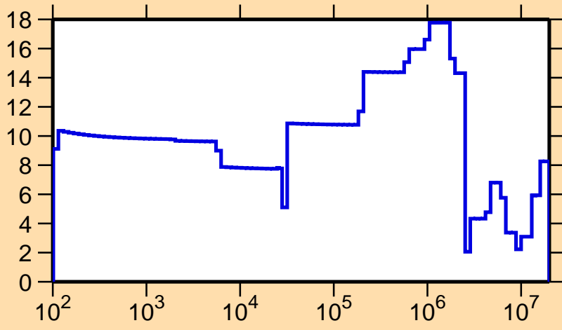
\Delta\sigma/\sigma vs. E for ^{91}\text{Tc}(n,el.)
