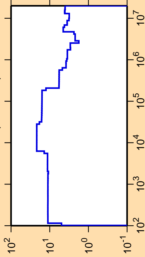
\Delta\sigma/\sigma vs. E for ^{91}\text{Tc}(n,\text{nonel.})
