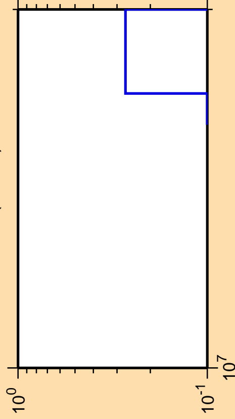
\Delta\sigma/\sigma vs. E for ^{91}\text{Tc} (mt 34)
