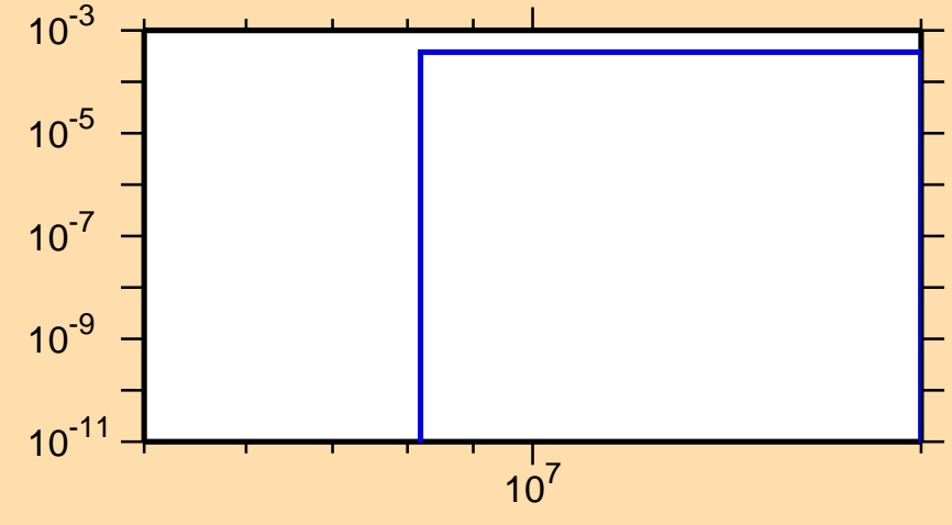
\sigma vs. E for ^{91}\text{Tc}(n,n\alpha)
