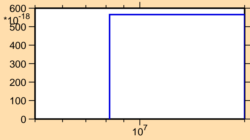
\sigma vs. E for ^{91}\text{Tc}(\text{mt } 34)
