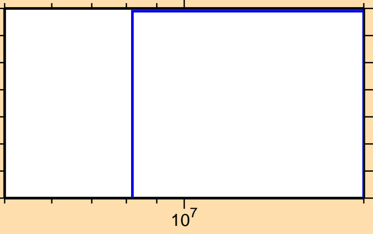
\sigma vs. E for ^{91}\text{Tc}(n,\text{nd})
