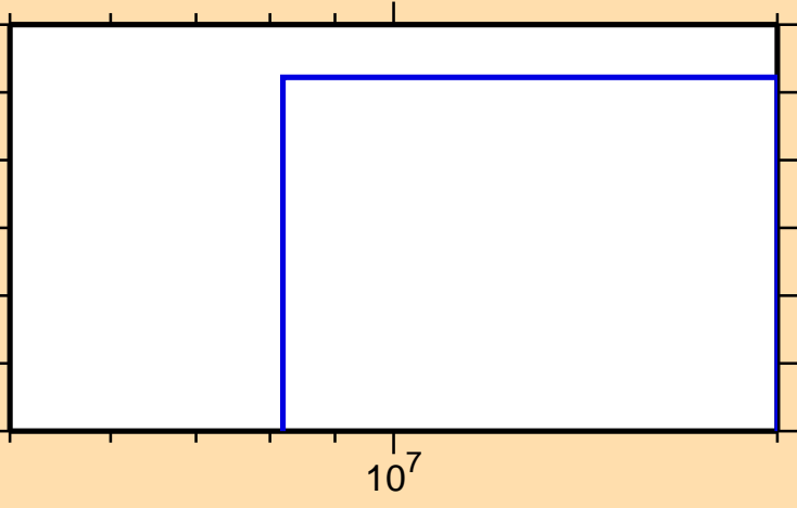
\sigma vs. E for ^{91}\text{Tc}(\text{mt } 45)
