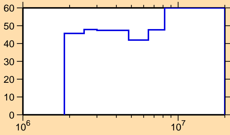
\Delta\sigma/\sigma vs. E for ^{91}\text{Tc}(n,ncont.)
