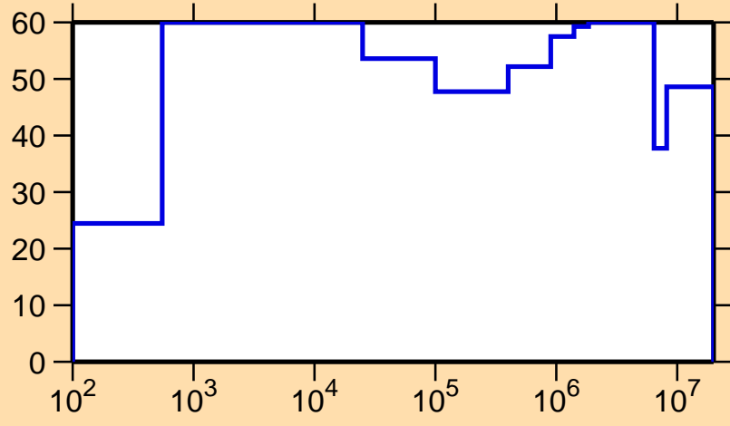
\Delta\sigma/\sigma vs. E for ^{91}\text{Tc}(n,\gamma)
