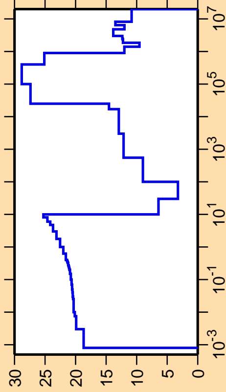
\Delta\sigma/\sigma vs. E for ^{91}\text{Tc}(n,\text{el.})
