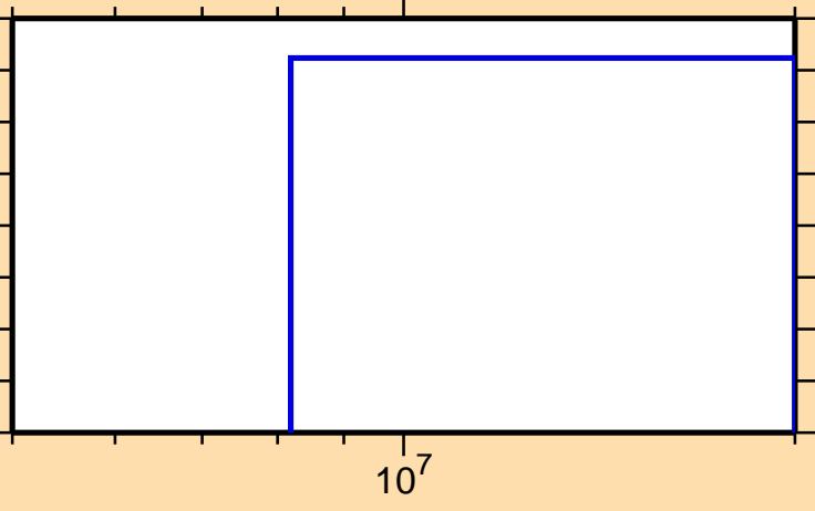
\sigma vs. E for ^{91}\text{Tc}(n,\text{nd})
