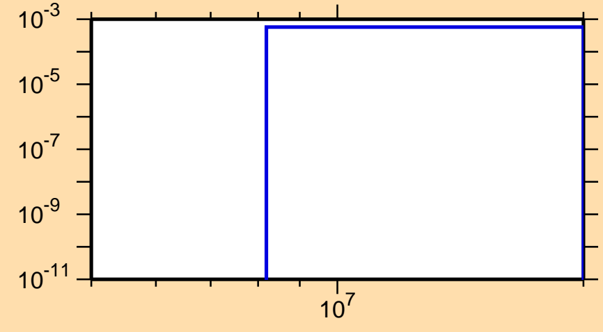
\sigma vs. E for ^{91}\text{Tc}(n,\alpha)
