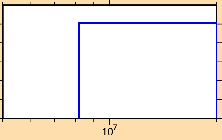
\sigma vs. E for ^{91}\text{Tc}(n,\text{pt})
