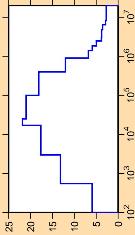
\Delta\sigma/\sigma vs. E for ^{92}\text{Tc}(n,\text{nonel.})
