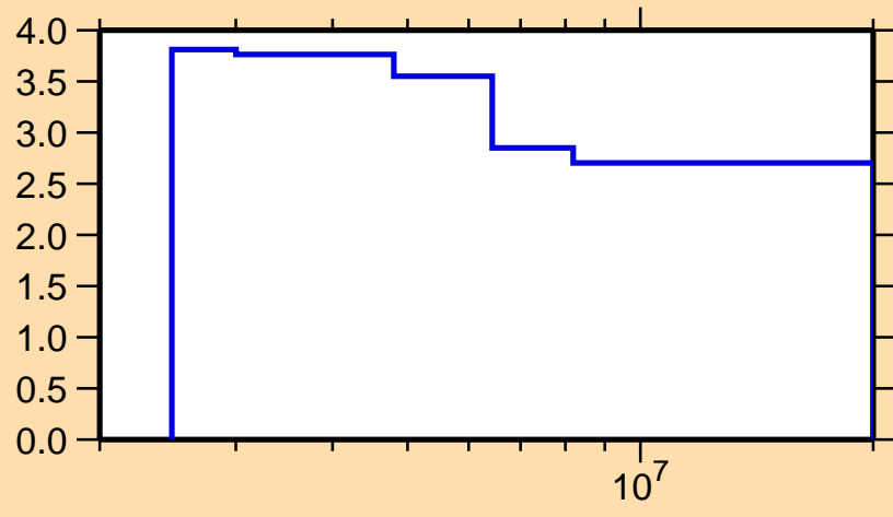
\Delta\sigma/\sigma vs. E for ^{92}\text{Tc}(n,n\text{onel.})
