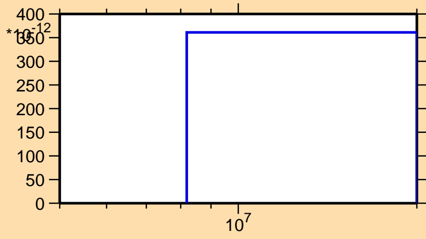
\sigma vs. E for ^{92}\text{Tc}(n,\text{pt})
