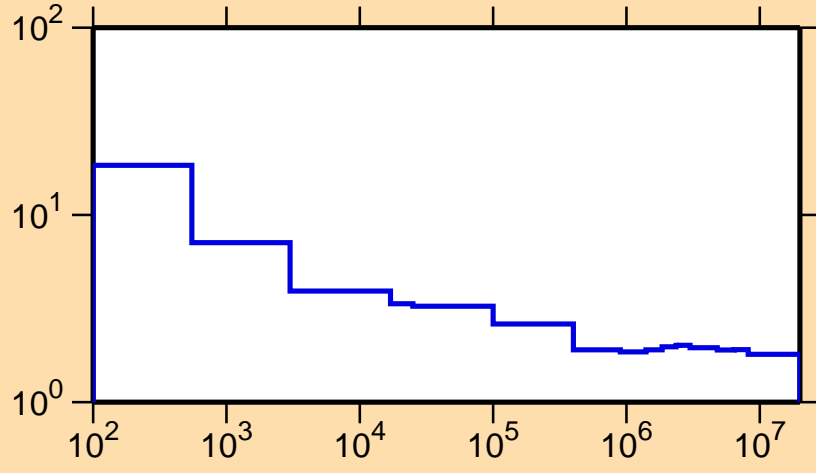
\sigma vs. E for ^{92}\text{Tc}(n,\text{nonel.})
