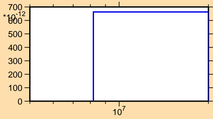
\sigma vs. E for ^{92}\text{Tc}(\text{mt } 45)
