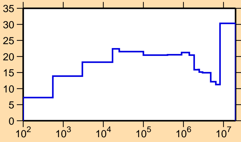
\Delta\sigma/\sigma vs. E for ^{92}\text{Tc}(n,p)
