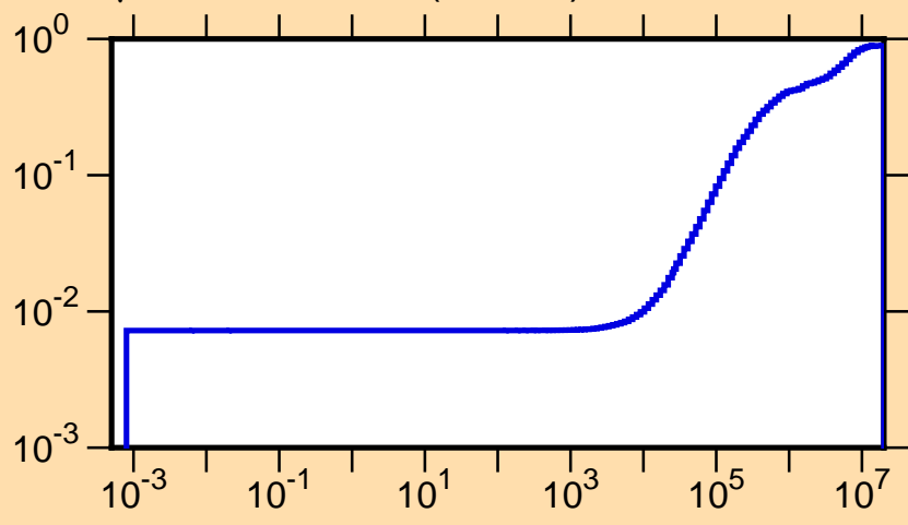
\mu vs. E for ^{93}\text{Tc}(\text{mt251})
