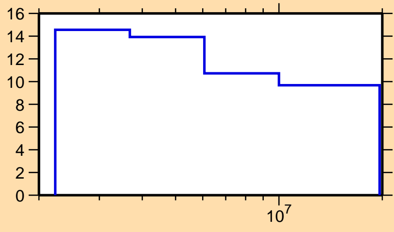
\Delta\sigma/\sigma vs. E for ^{93}\text{Tc}(n,n\text{onel.})
