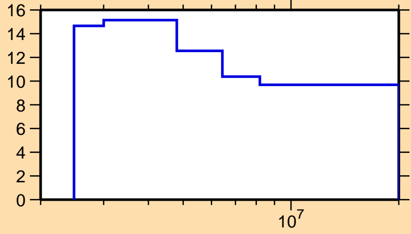
\Delta\sigma/\sigma vs. E for ^{93}\text{Tc}(n,n\text{nonel.})
