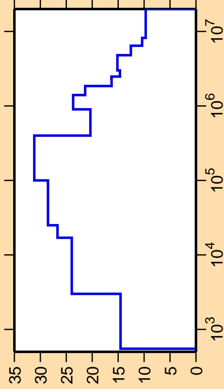
\Delta\sigma/\sigma vs. E for ^{93}\text{Tc}(n,\text{nonel.})
