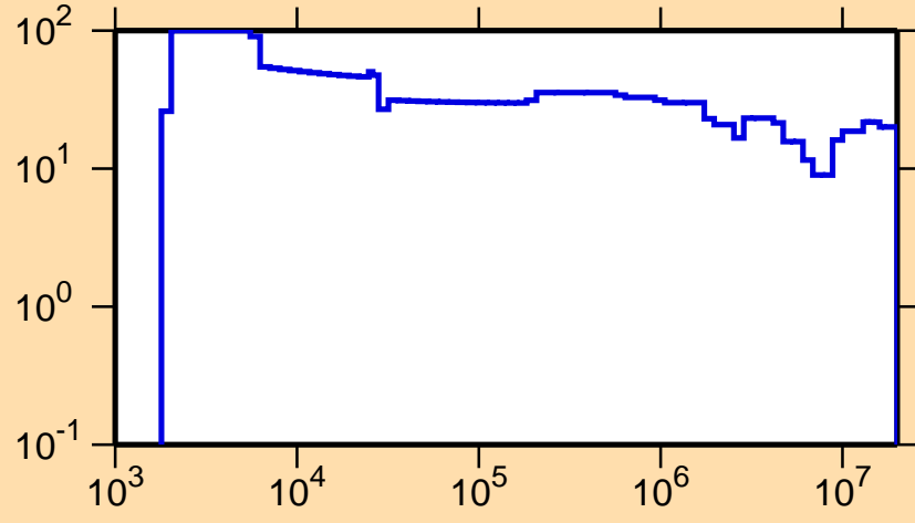
\Delta\sigma/\sigma vs. E for ^{93}\text{Tc}(n,el.)
