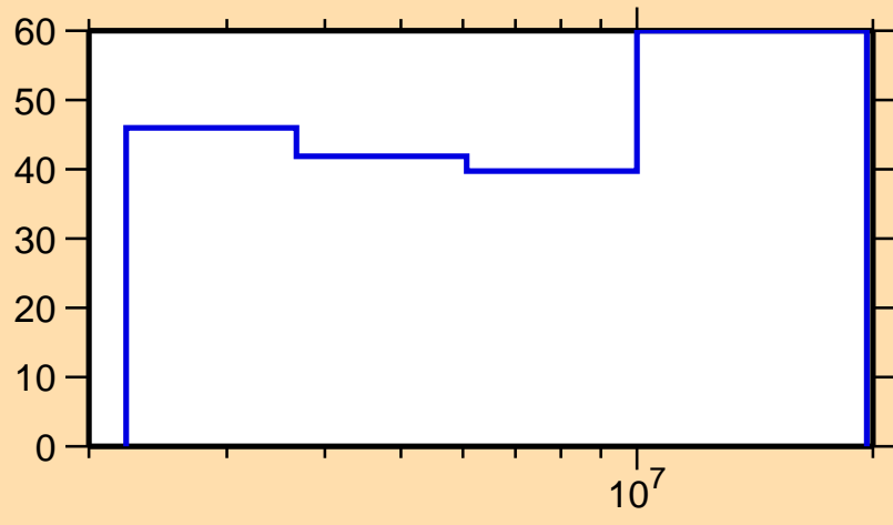
\Delta\sigma/\sigma vs. E for ^{93}\text{Tc}(n,n\text{cont.})
