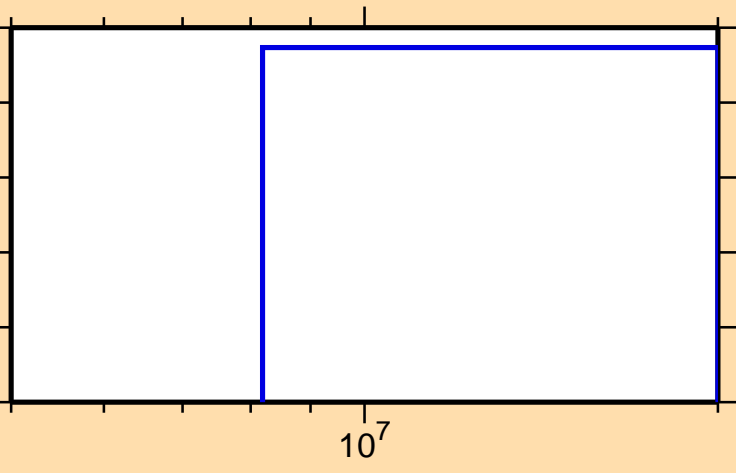
\sigma vs. E for ^{93}\text{Tc}(n,\text{pd})
