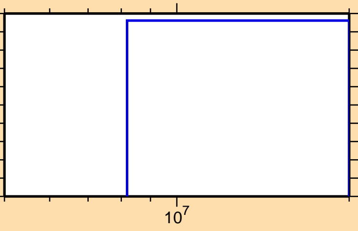
\sigma vs. E for ^{93}\text{Tc}(n,t)
