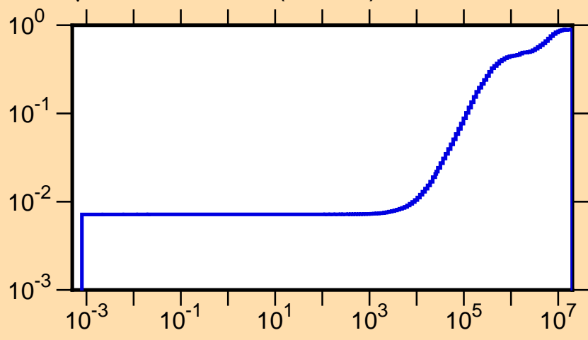
\mu vs. E for ^{94}\text{Tc}(\text{mt251})
