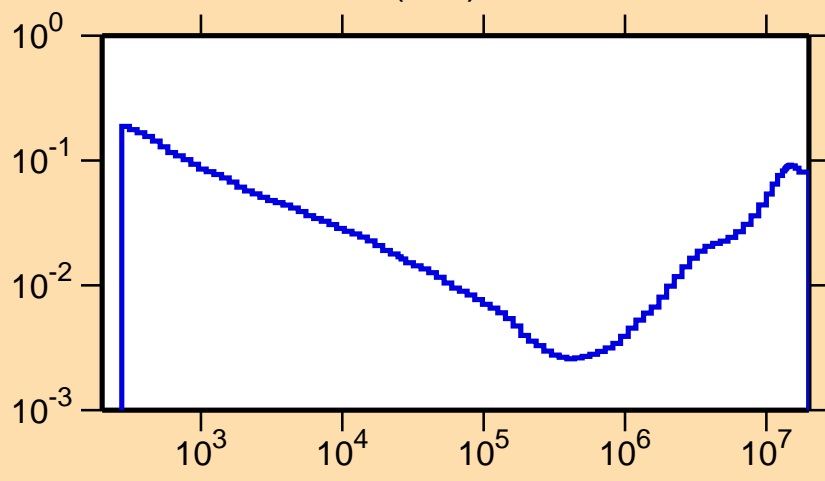
\sigma vs. E for ^{94}\text{Tc}(n,\alpha)
