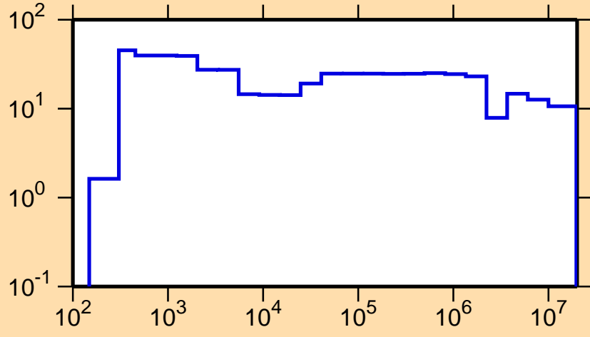
\Delta\sigma/\sigma vs. E for ^{94}\text{Tc}(n,el.)
