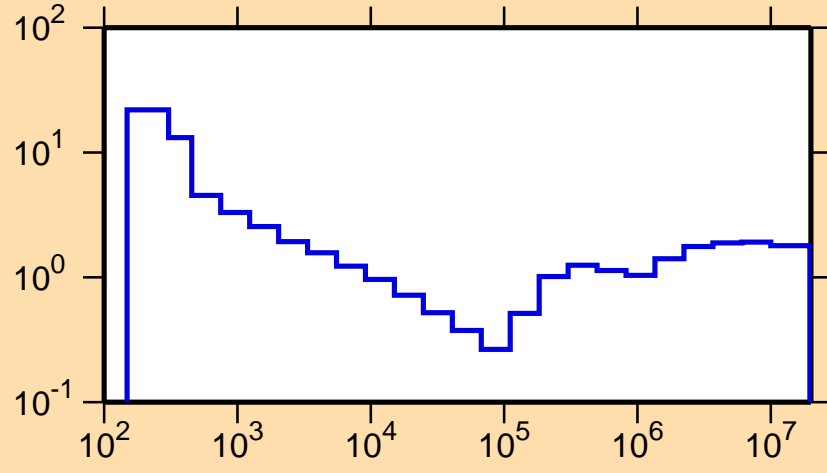
\sigma vs. E for ^{94}\text{Tc}(n,\text{nonel.})
