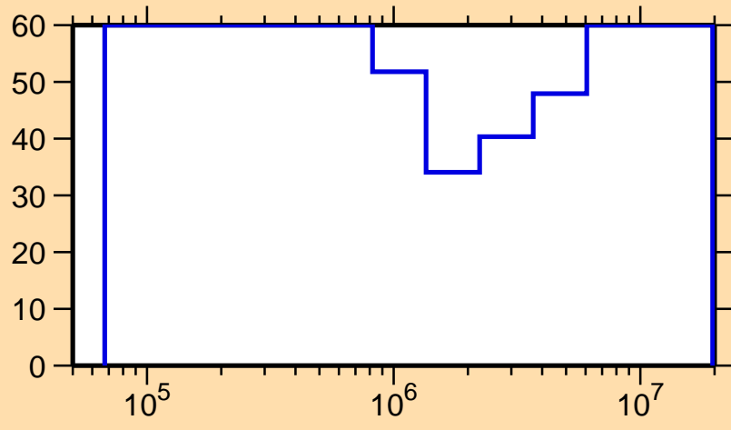
\Delta\sigma/\sigma vs. E for ^{94}\text{Tc}(n,n_1)
