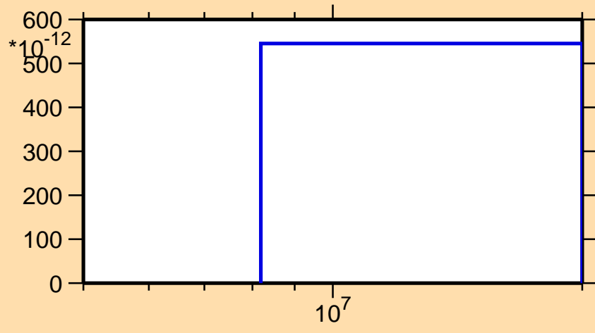
\sigma vs. E for ^{94}\text{Tc}(\text{mt } 45)
