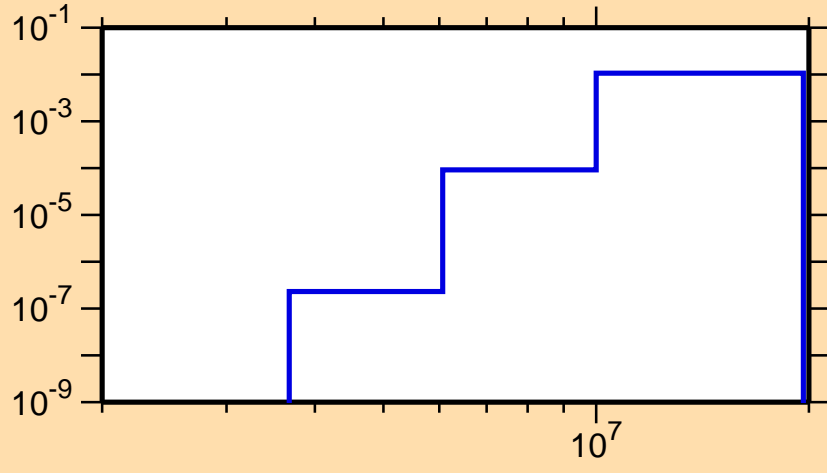
\sigma vs. E for ^{94}\text{Tc}(n,p\alpha)
