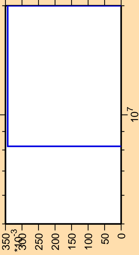
\Delta\sigma/\sigma vs. E for ^{94}\text{Tc}(n,nt)
