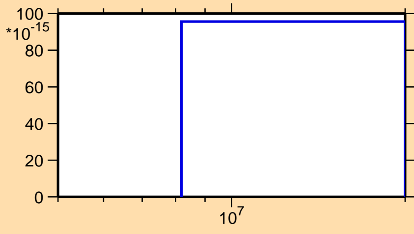
\sigma vs. E for ^{94}\text{Tc}(n,nt)
