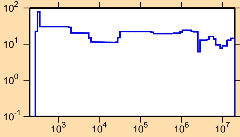
\Delta\sigma/\sigma vs. E for ^{95}\text{Tc}(n,el.)
