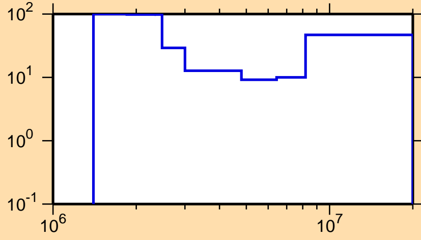
\Delta\sigma/\sigma vs. E for ^{95}\text{Tc}(n,n\text{cont.})
