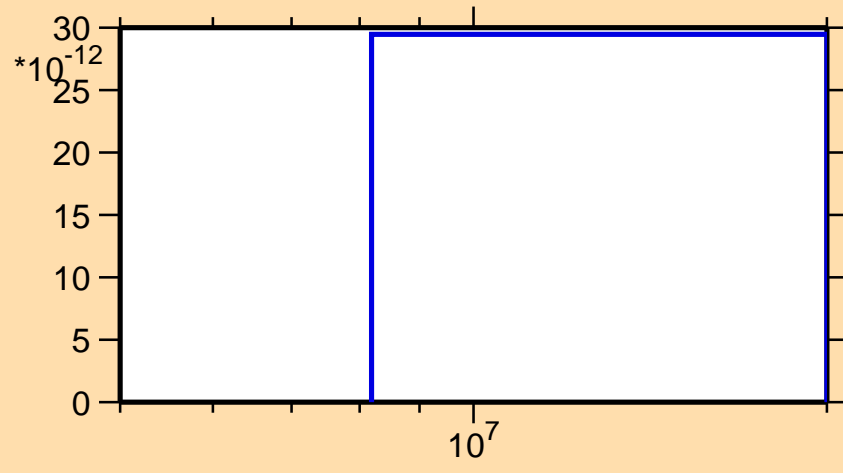
\sigma vs. E for ^{95}\text{Tc}(n,2n\alpha)
