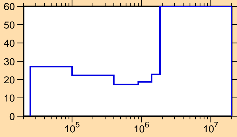
\Delta\sigma/\sigma vs. E for ^{95}\text{Tc}(n,n_1)
