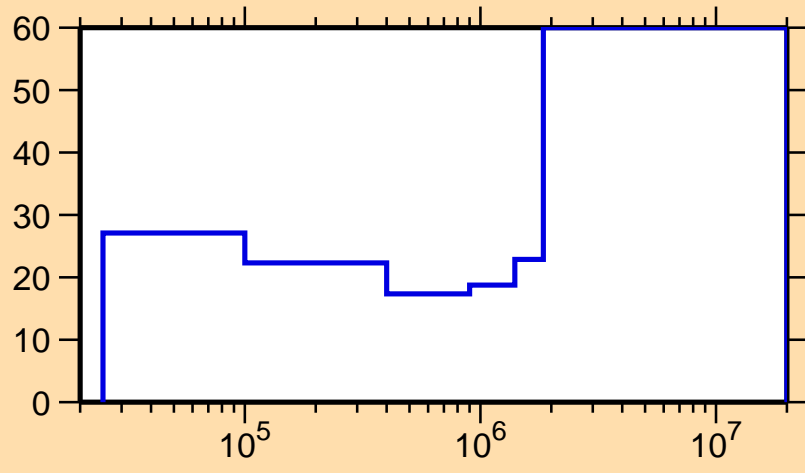
\Delta\sigma/\sigma vs. E for ^{95}\text{Tc}(n,n_1)
