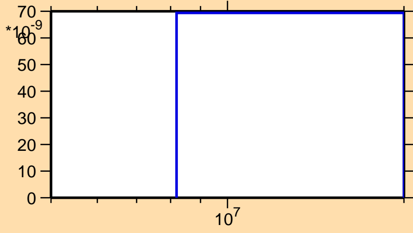
\sigma vs. E for ^{95}\text{Tc}(\text{mt } 45)
