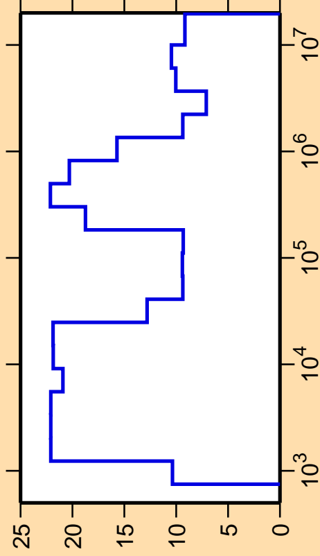
\Delta\sigma/\sigma vs. E for ^{95}\text{Tc}(n,\text{nonel.})
