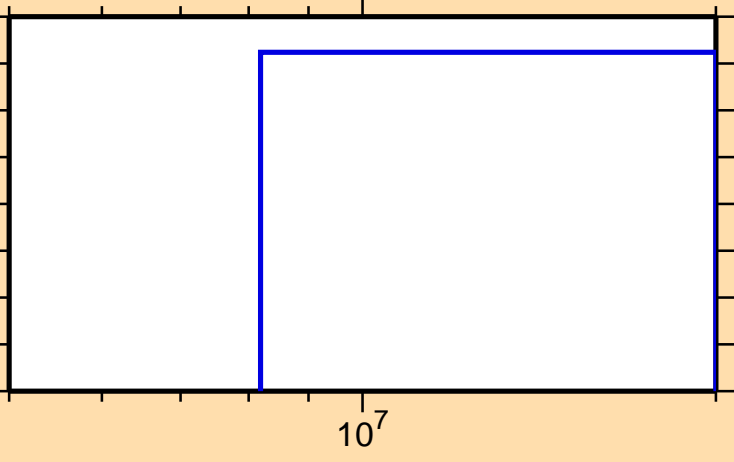
\sigma vs. E for ^{95}\text{Tc}(n,2n\alpha)
