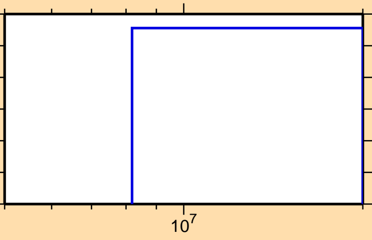
\sigma vs. E for ^{95}\text{Tc}(n,nt)
