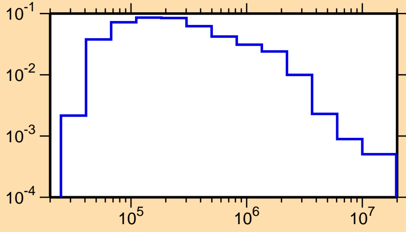
\sigma vs. E for ^{96}\text{Tc}(n,n_1)
