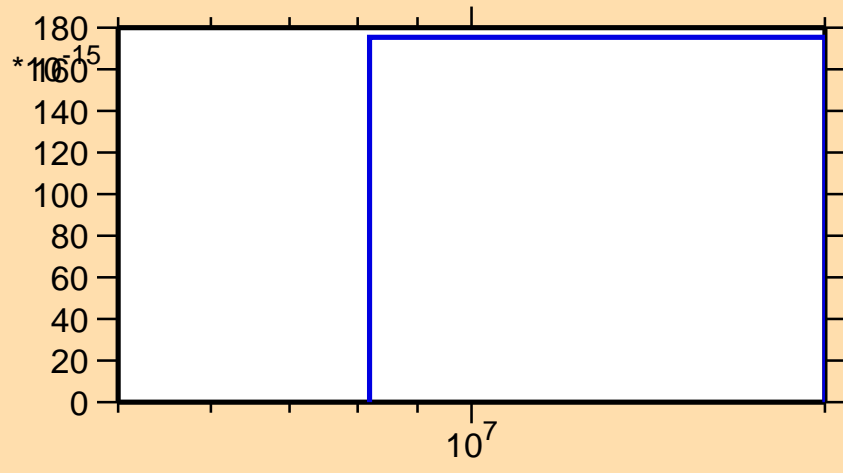
\sigma vs. E for ^{96}\text{Tc}(\text{mt } 34)
