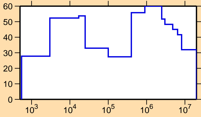
\Delta\sigma/\sigma vs. E for ^{96}\text{Tc}(n,p)
