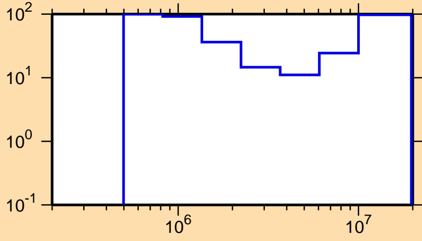
\Delta\sigma/\sigma vs. E for ^{96}\text{Tc}(n,ncont.)
