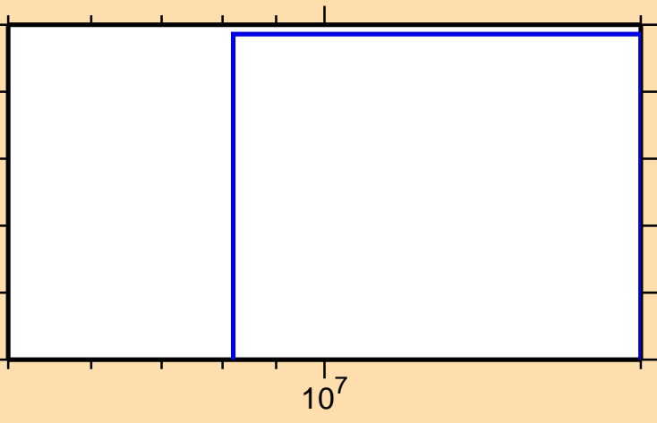
\sigma vs. E for ^{96}\text{Tc}(\text{mt117})
