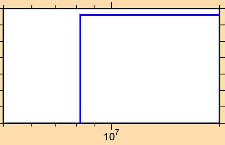
\sigma vs. E for ^{96}\text{Tc}(n,\text{nd})
