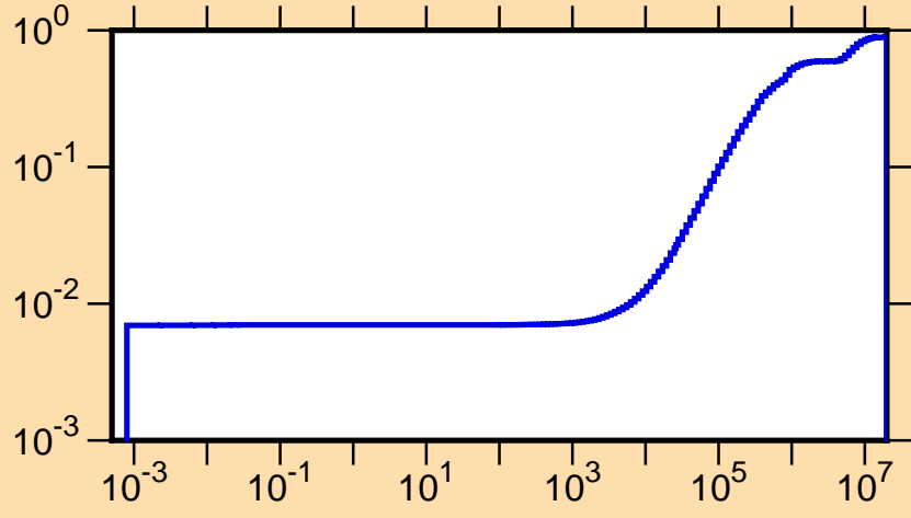
\mu vs. E for ^{97}\text{Tc}(\text{mt251})
