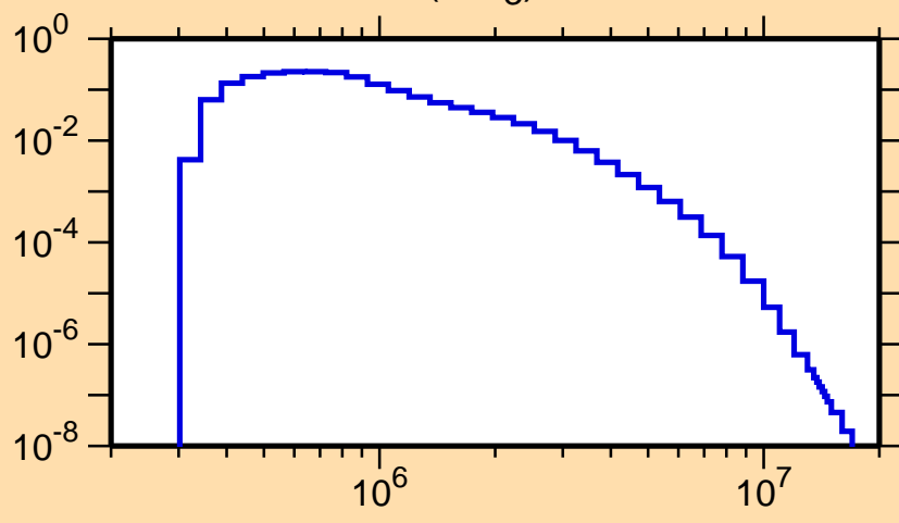
\sigma vs. E for ^{97}\text{Tc}(n,n_3)
