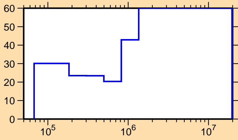
\Delta\sigma/\sigma vs. E for ^{97}\text{Tc}(n,n_1)
