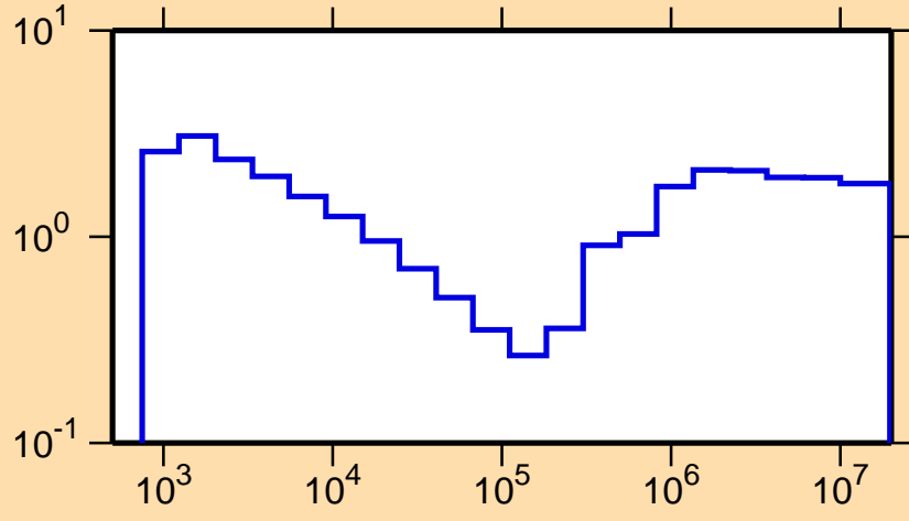
\sigma vs. E for ^{97}\text{Tc}(n,\text{nonel.})
