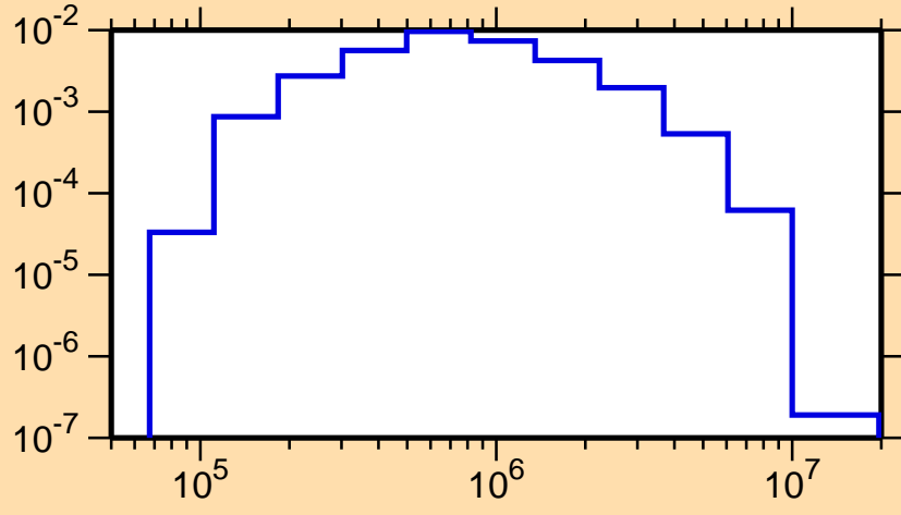
\sigma vs. E for ^{97}\text{Tc}(n,n_1)
