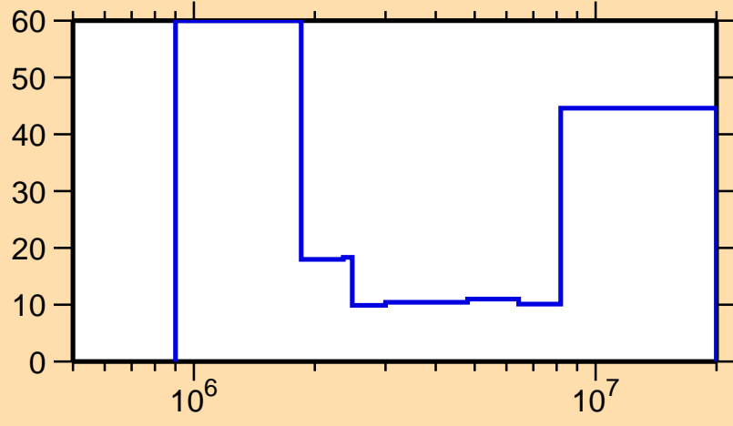
\Delta\sigma/\sigma vs. E for ^{97}\text{Tc}(n,n\text{cont.})
