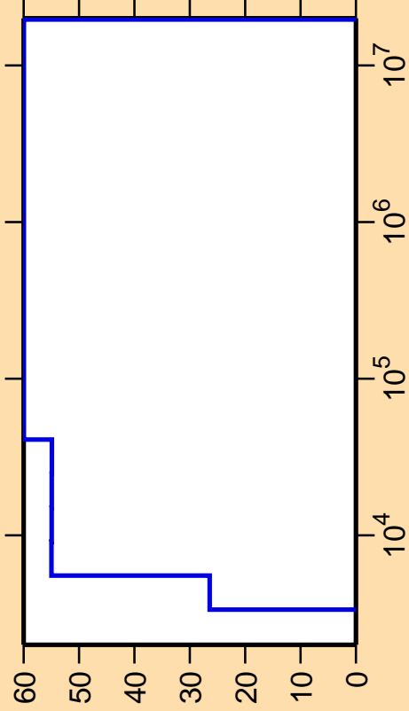
\Delta\sigma/\sigma vs. E for ^{98}\text{Tc}(n,p)
