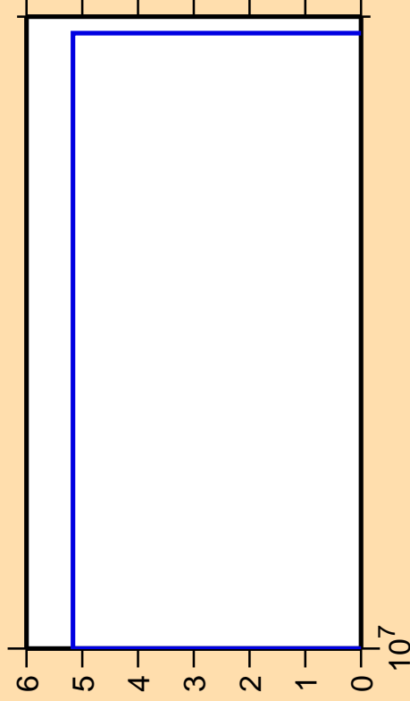
\Delta\sigma/\sigma vs. E for ^{98}\text{Tc} (mt 45)
