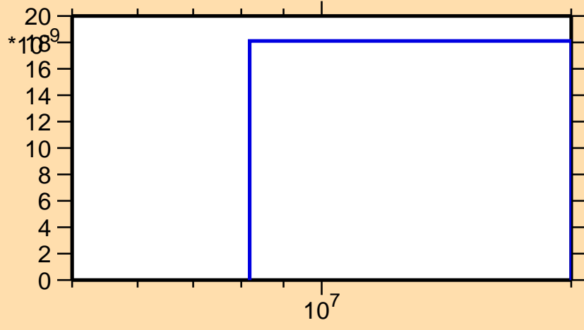
\sigma vs. E for ^{98}\text{Tc}(n,\text{He}3)
