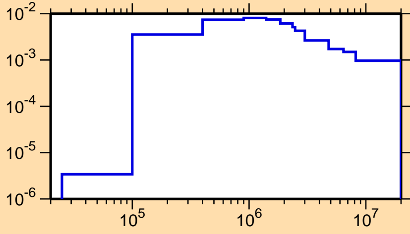
\sigma vs. E for ^{98}\text{Tc}(n,n_3)
