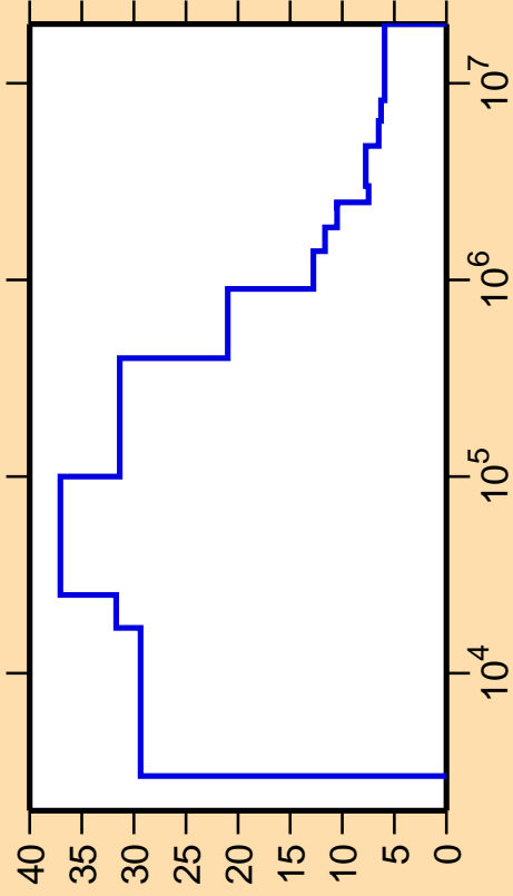
\Delta\sigma/\sigma vs. E for ^{98}\text{Tc}(n,\text{nonel.})
