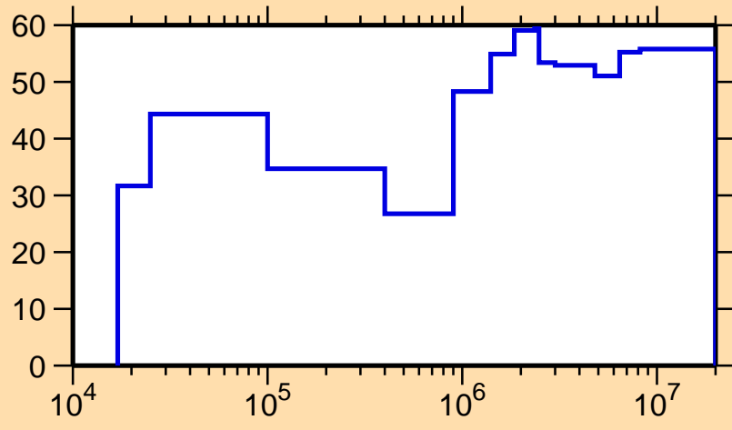
\Delta\sigma/\sigma vs. E for ^{98}\text{Tc}(n,n_1)
