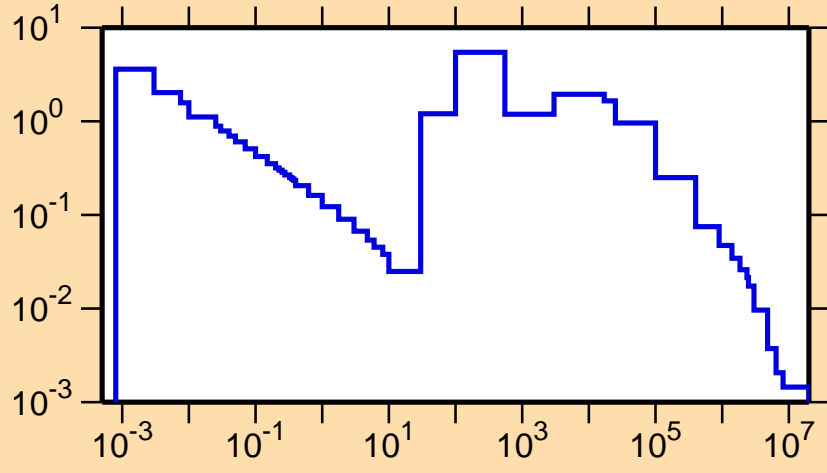
\sigma vs. E for ^{98}\text{Tc}(n,\gamma)
