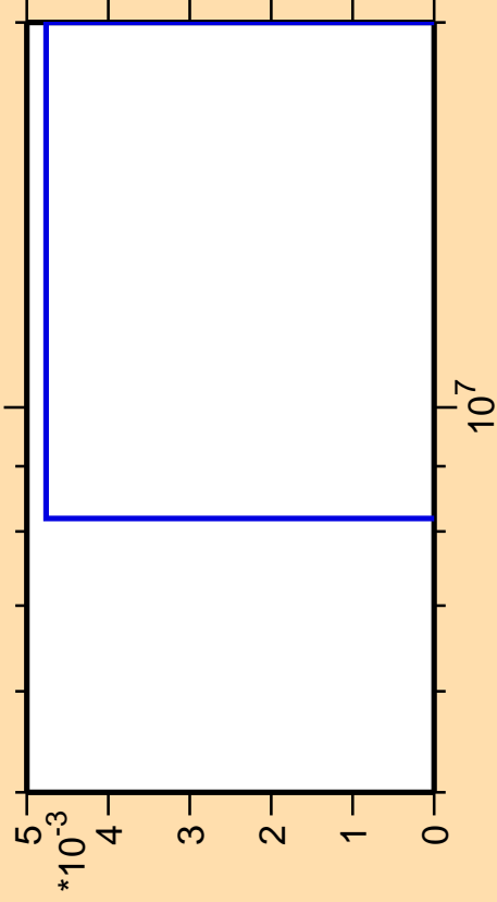
\Delta\sigma/\sigma vs. E for ^{98}\text{Tc} (mt 34)
