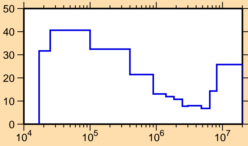
\Delta\sigma/\sigma vs. E for ^{98}\text{Tc}(n,\text{inel.})
