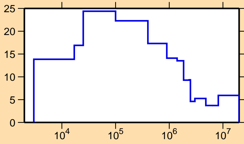
\Delta\sigma/\sigma vs. E for ^{98}\text{Tc}(n,\text{tot.})
