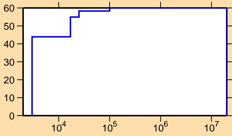
\Delta\sigma/\sigma vs. E for ^{98}\text{Tc}(n,p)
