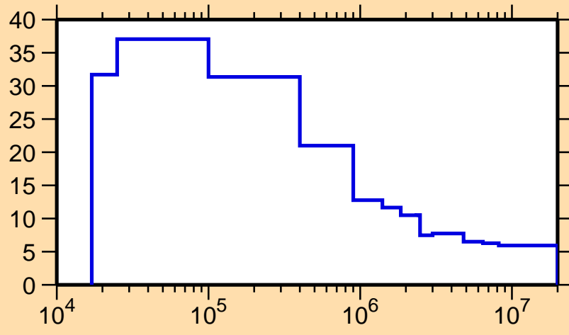
\Delta\sigma/\sigma vs. E for ^{98}\text{Tc}(n,\text{nonel.})
