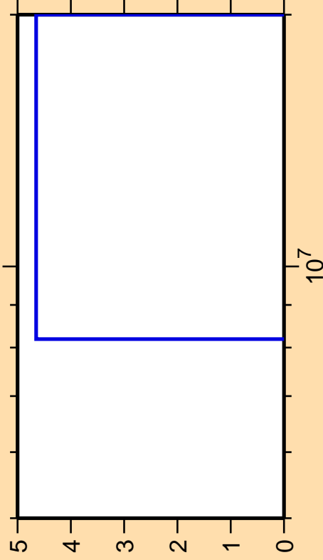
\Delta\sigma/\sigma vs. E for ^{98}\text{Tc}(\text{mt } 45)
