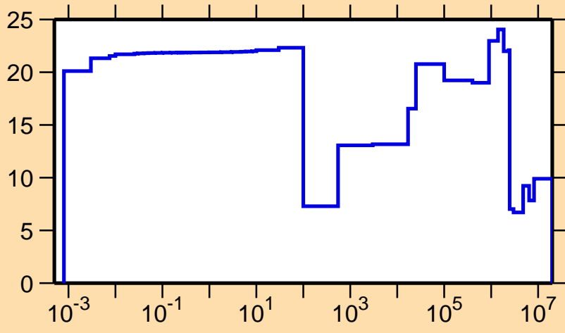
\Delta\sigma/\sigma vs. E for ^{98}\text{Tc}(n,\text{el.})
