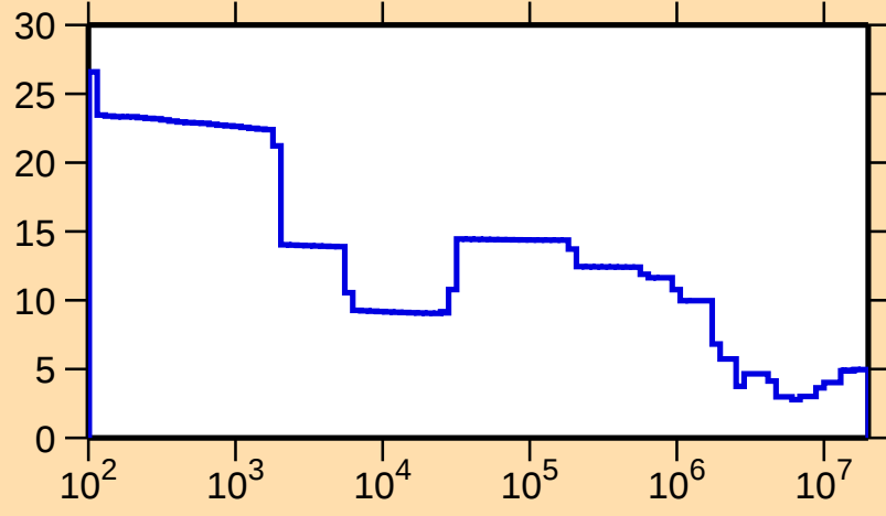
\Delta\sigma/\sigma vs. E for ^{99}\text{Tc}(n,\text{tot.})
