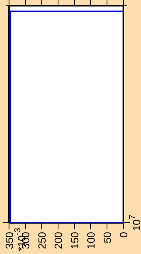
\Delta\sigma/\sigma vs. E for ^{99}\text{Tc}(\text{mt } 45)
