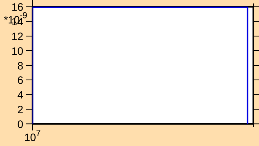
\sigma vs. E for ^{99}\text{Tc}(n,\text{nt})
