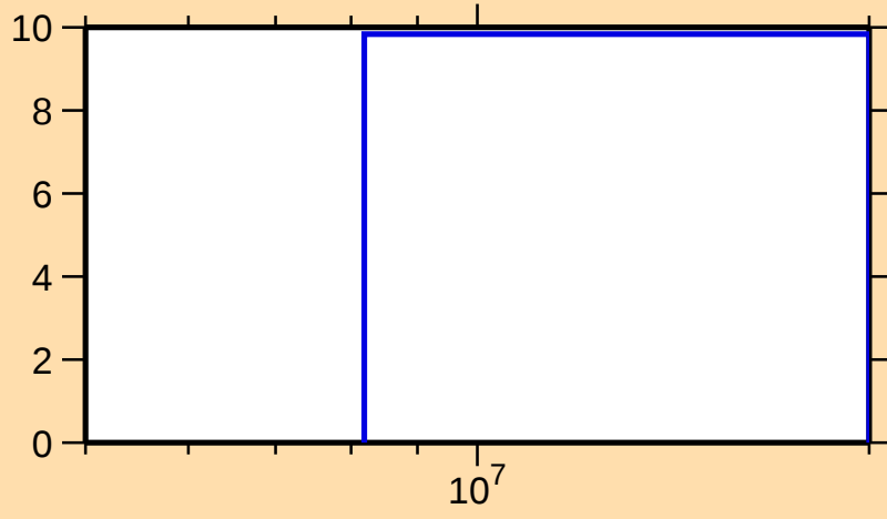
\Delta\sigma/\sigma vs. E for ^{99}\text{Tc}(n,2n)
