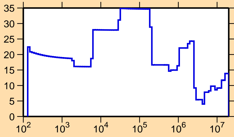
\Delta\sigma/\sigma vs. E for ^{100}\text{Tc}(n,el.)
