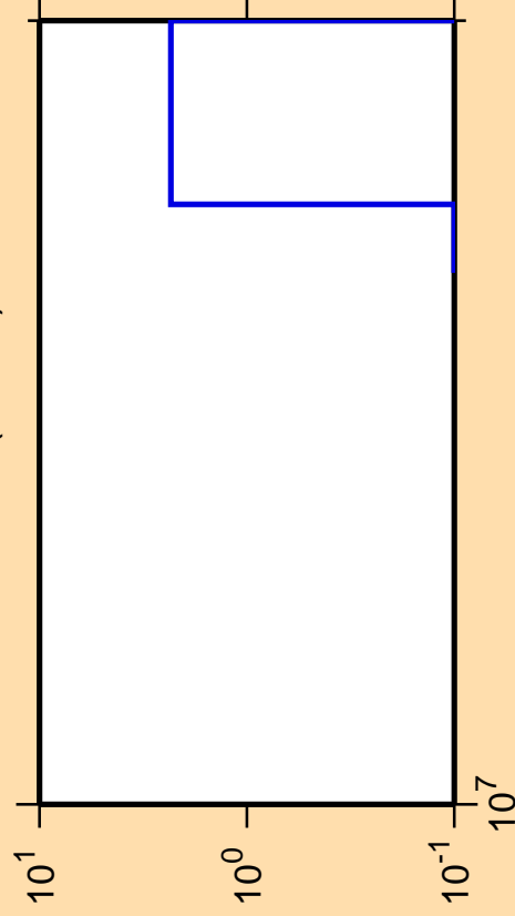
\Delta\sigma/\sigma vs. E for ^{100}\text{Tc} (mt 45)
