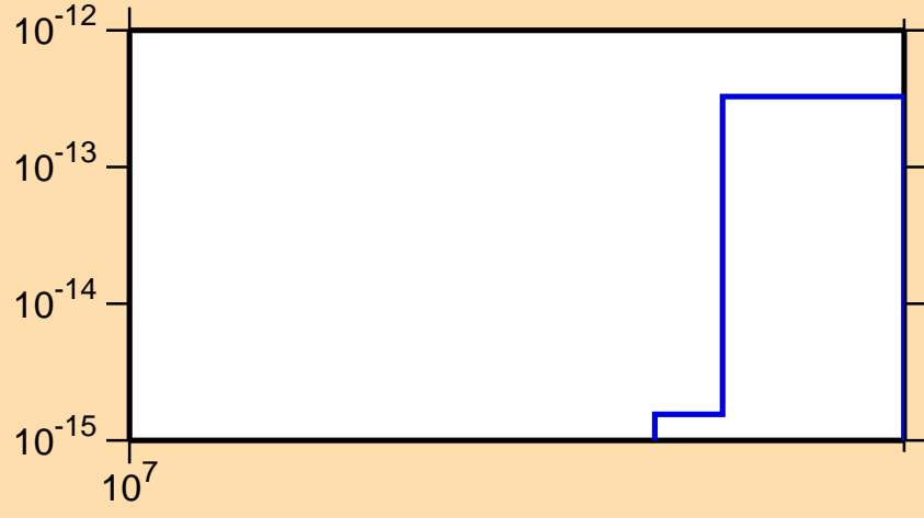
\sigma vs. E for ^{100}\text{Tc} (mt 45)
