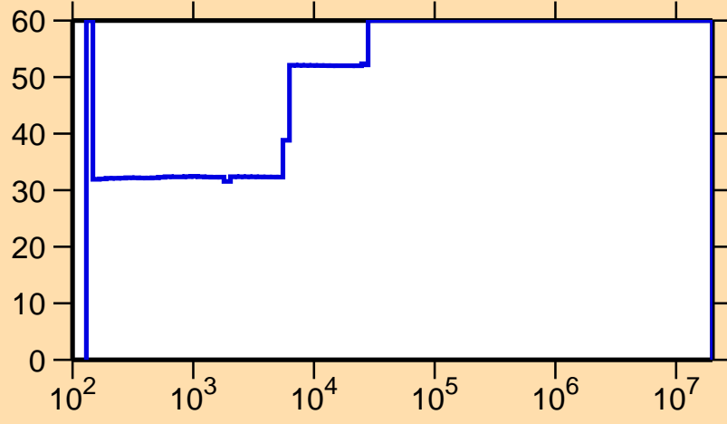
\Delta\sigma/\sigma vs. E for ^{100}\text{Tc}(n,\gamma)
