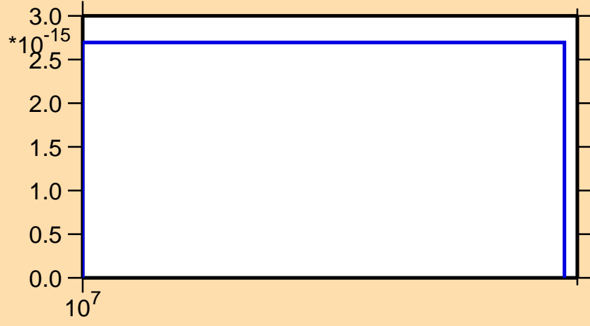
\sigma vs. E for ^{100}\text{Tc} (mt 45)
