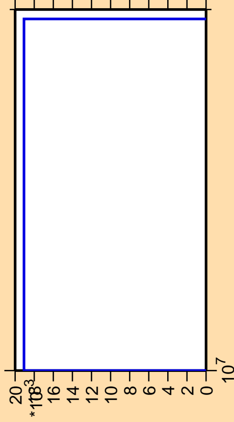
\Delta\sigma/\sigma vs. E for ^{100}\text{Tc} (mt 45)
