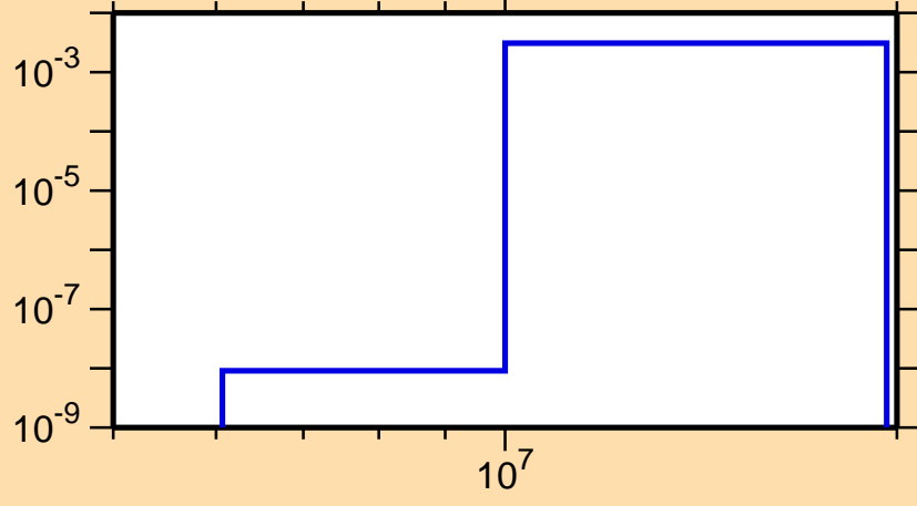
\sigma vs. E for ^{100}\text{Tc}(n,np)
