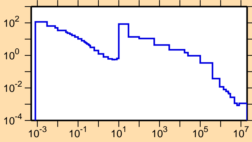
\sigma vs. E for ^{100}\text{Tc}(n,\gamma)
