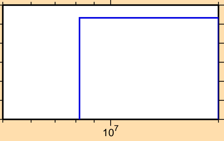
\sigma vs. E for ^{100}\text{Tc}(n,\text{He3})
