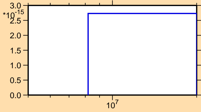
\sigma vs. E for ^{100}\text{Tc}(\text{mt } 45)
