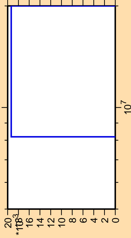
\Delta\sigma/\sigma vs. E for ^{100}\text{Tc}(\text{mt } 45)
