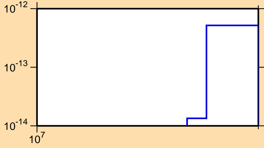
\sigma vs. E for ^{101}\text{Tc}(\text{mt117})
