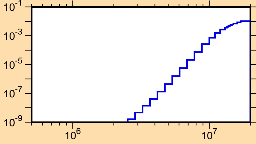
\sigma vs. E for ^{101}\text{Tc}(n,\alpha)
