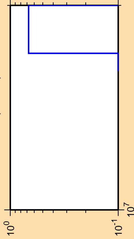
\Delta\sigma/\sigma vs. E for ^{101}\text{Tc}(\text{mt117})
