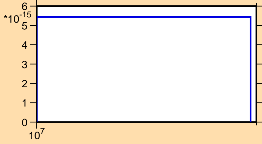
\sigma vs. E for ^{101}\text{Tc}(\text{mt117})
