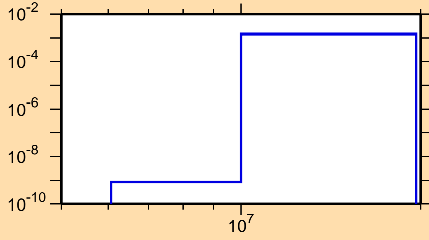
\sigma vs. E for ^{101}\text{Tc}(n,np)
