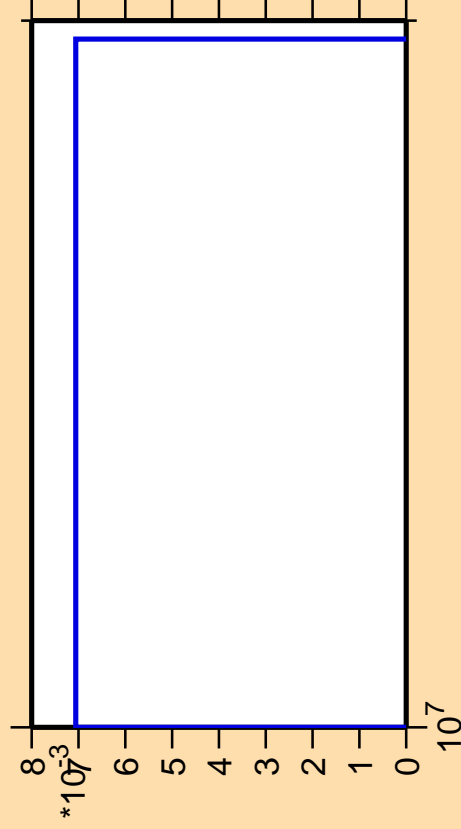
\Delta\sigma/\sigma vs. E for ^{101}\text{Tc}(\text{mt117})
