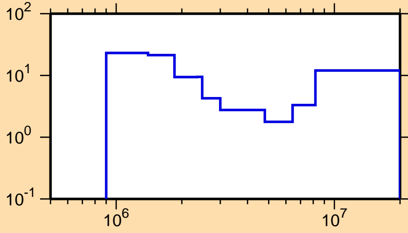
\Delta\sigma/\sigma vs. E for ^{101}\text{Tc}(n,n\text{cont.})
