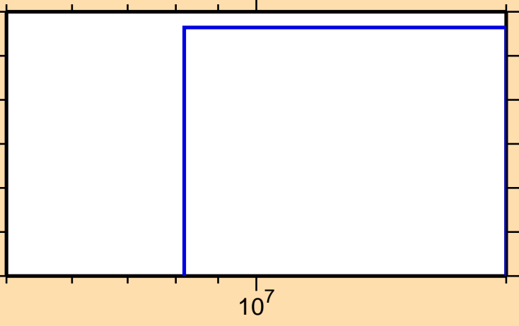
\sigma vs. E for ^{101}\text{Tc}(n,\text{nd})
