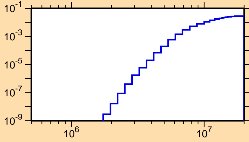
\sigma vs. E for ^{102}\text{Tc}(n,p)
