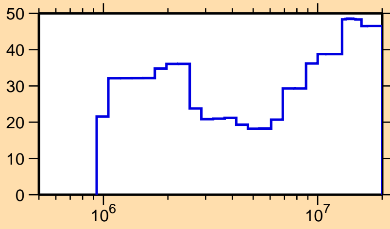
\Delta\sigma/\sigma vs. E for ^{102}\text{Tc}(n,\gamma)
