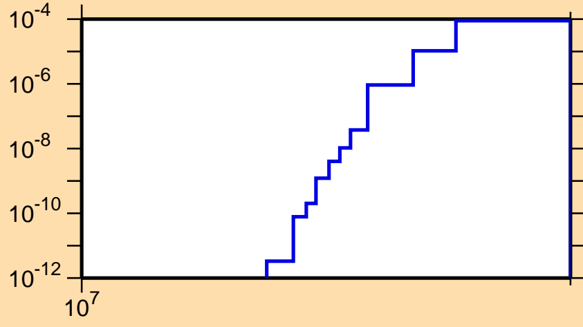
\sigma vs. E for ^{102}\text{Tc}(n,\text{nd})
