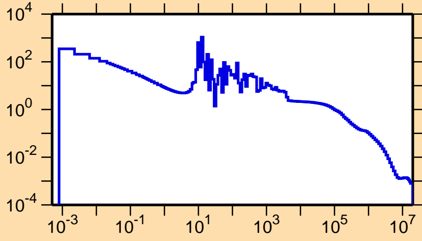
\sigma vs. E for ^{102}\text{Tc}(n,\gamma)
