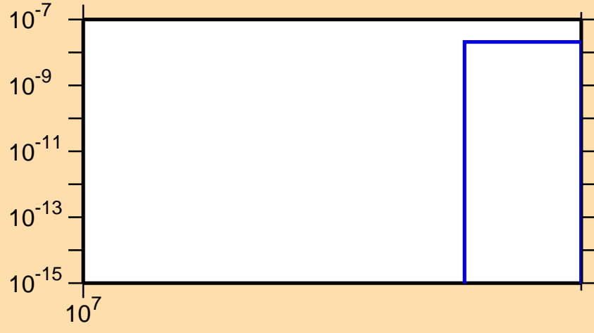
\sigma vs. E for ^{103}\text{Tc}(n,2np)
