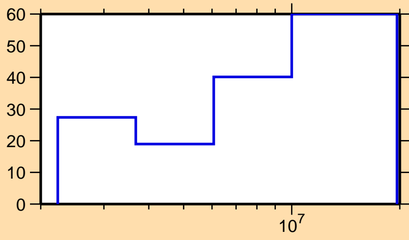
\Delta\sigma/\sigma vs. E for ^{103}\text{Tc}(n,n\text{cont.})
