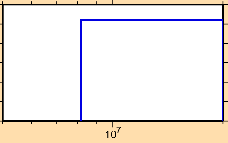
\sigma vs. E for ^{103}\text{Tc}(n,np)
