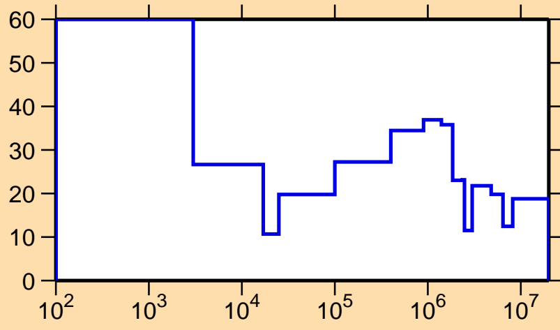
\Delta\sigma/\sigma vs. E for ^{103}\text{Tc}(n,\text{el.})
