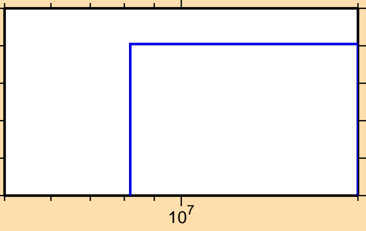
\sigma vs. E for ^{103}\text{Tc}(n,n\alpha)
