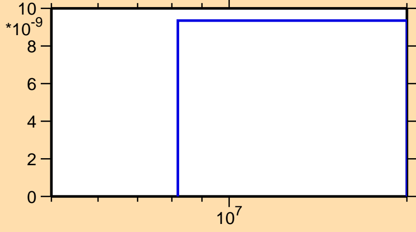
\sigma vs. E for ^{103}\text{Tc}(n,nt)
