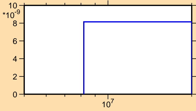
\sigma vs. E for ^{103}\text{Tc}(n,\text{nd})
