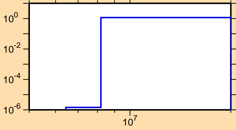
\sigma vs. E for ^{103}\text{Tc}(n,2n)
