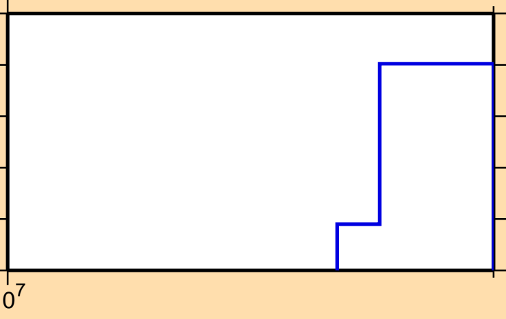
\sigma vs. E for ^{104}\text{Tc}(n,nt)
